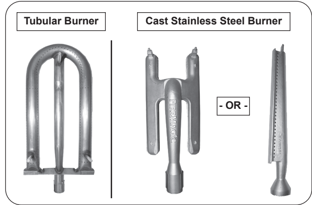
Fig. 4-1 Burner types
